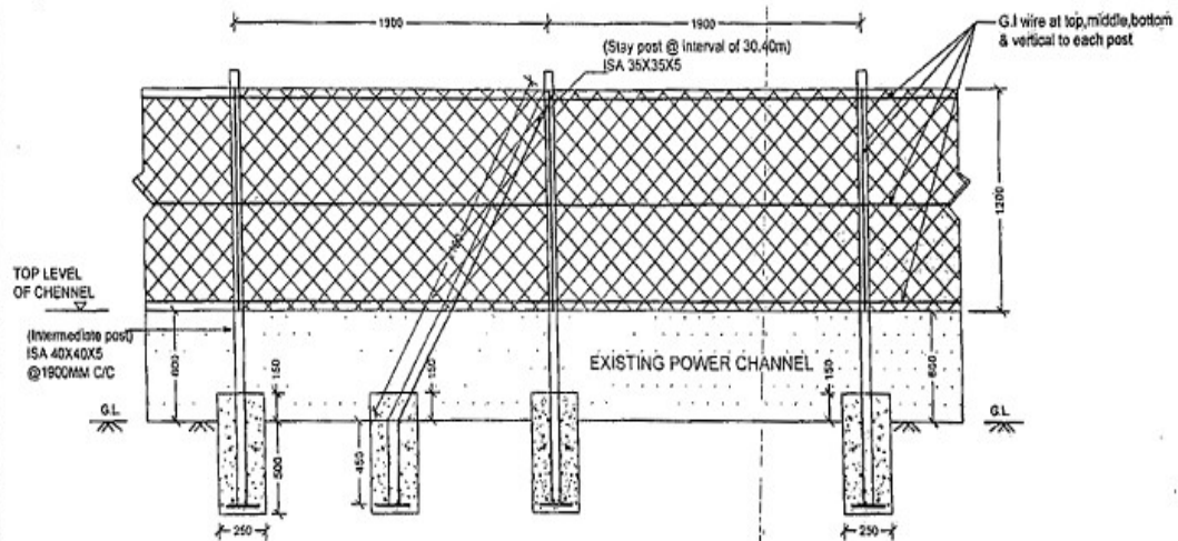
DETAIL OF STAY POST (@ INTERVAL OF 30.40M) AND INTERMEDIATE POST
