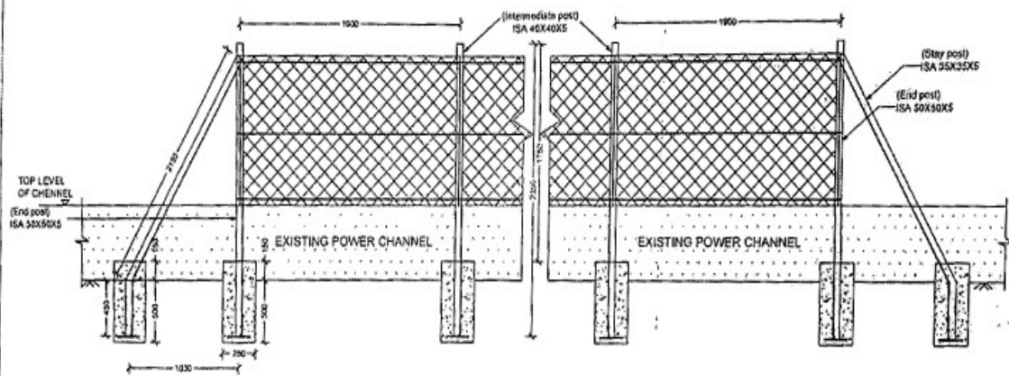
DETAIL OF END POST, INTERMEDIATE POST & STAY POST OF FENCING
